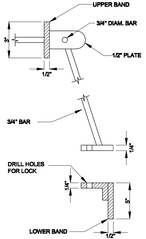
ENTRY GATE DETAIL
