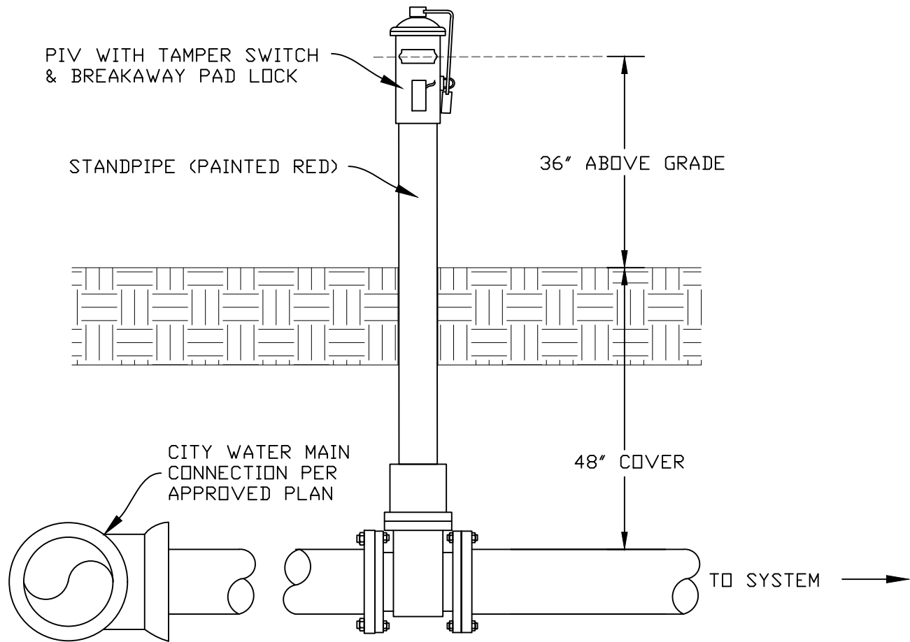
POST INDICATOR VALVE (PIV)
