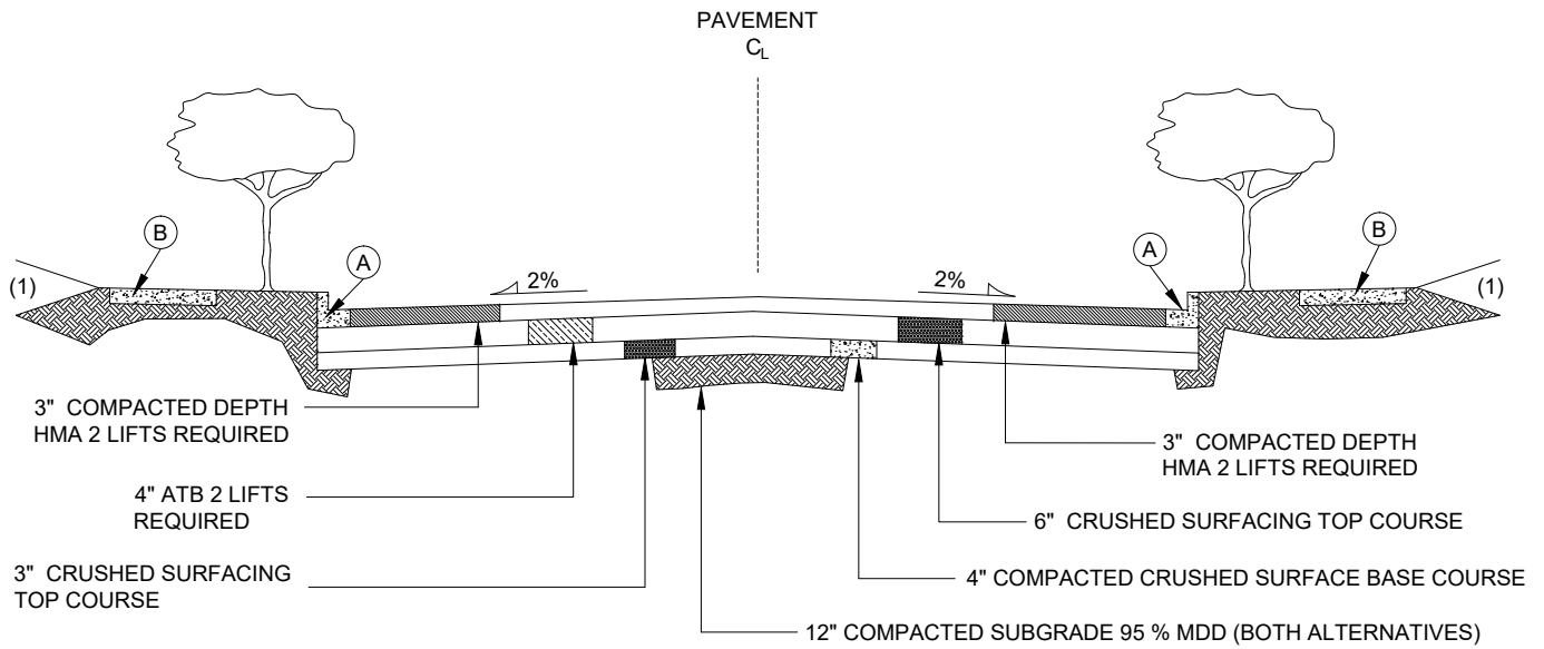
ALTERNATE PAVEMENT SECTION
