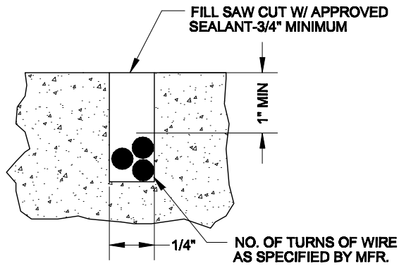
SECT. A-A
