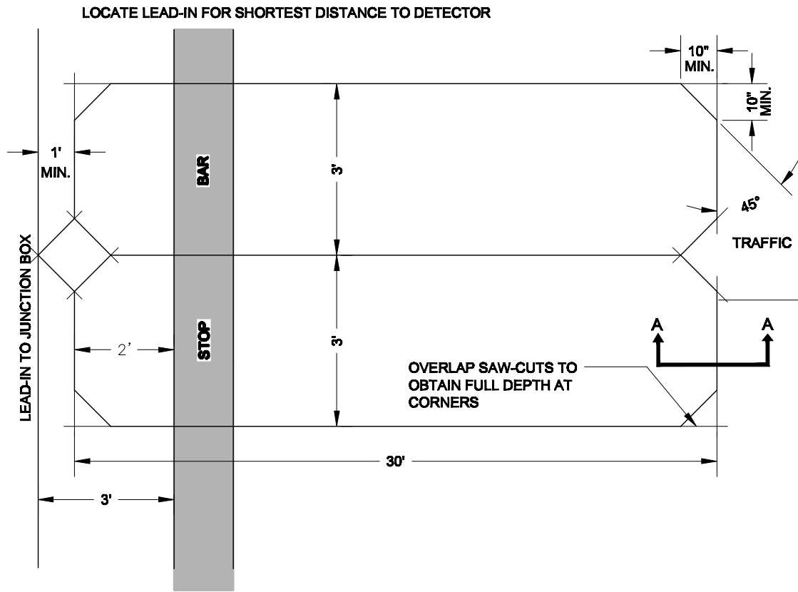
TYPICAL SAW CUT PLAN
