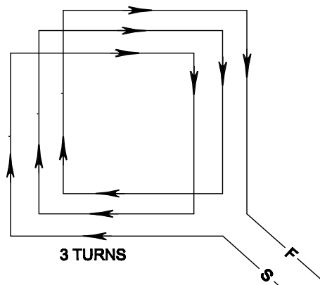
LOOP WINDING DETAIL
